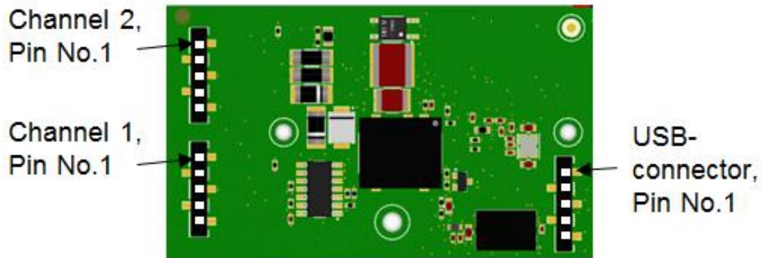
Figure 3-1: Displays (LED) on bottom side
