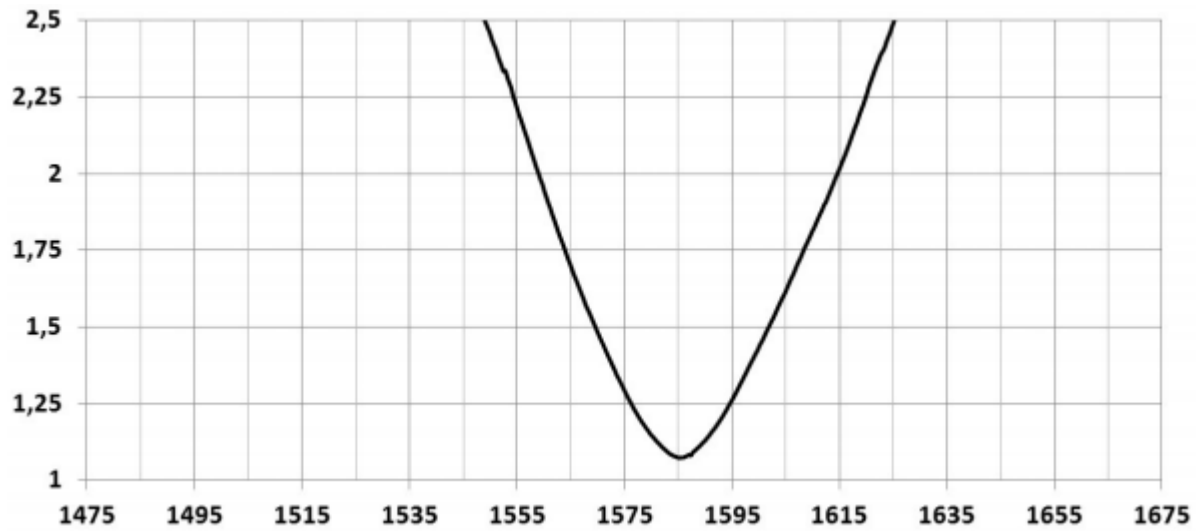
Antenna VSWR
