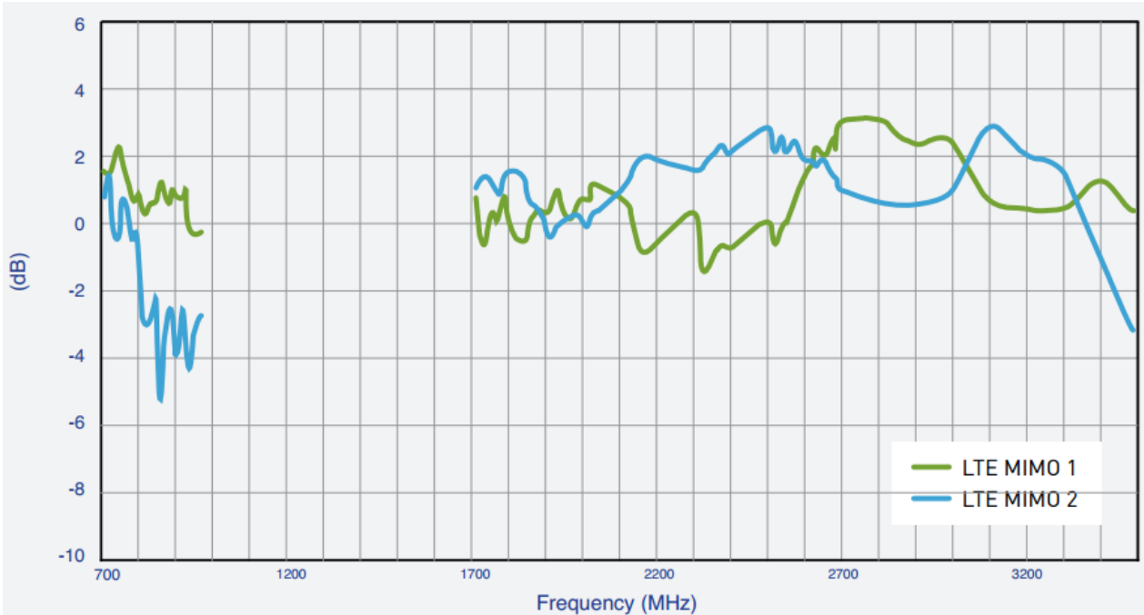
Maximum Gain
