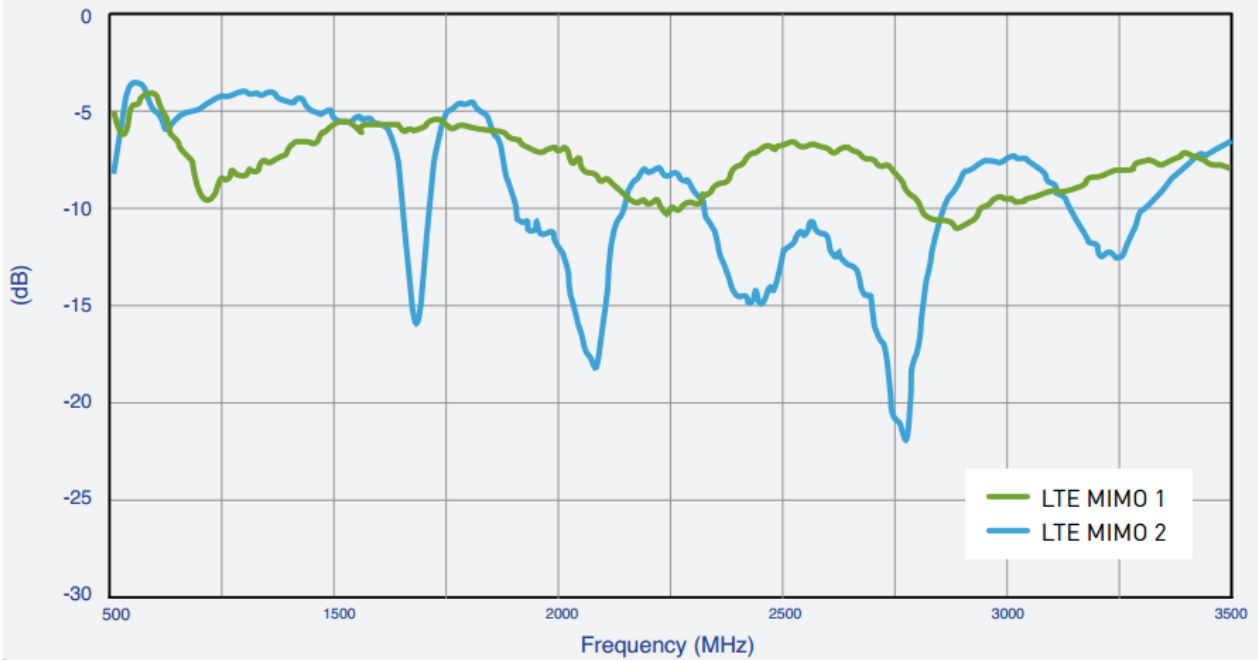
Return Loss
