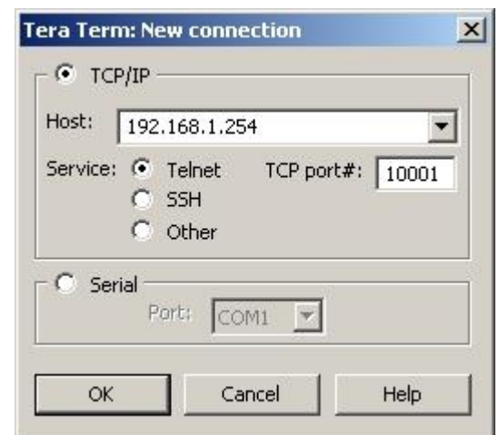
Fig. 28 – New connection
