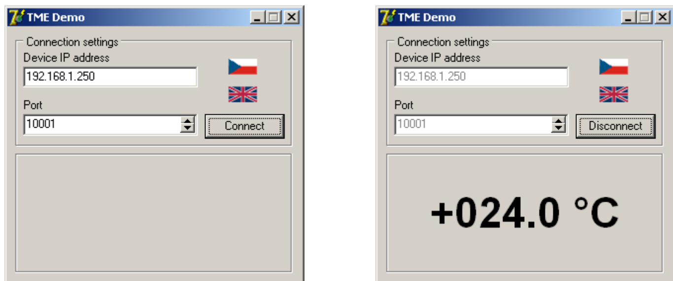
Fig. 29 – demo program
