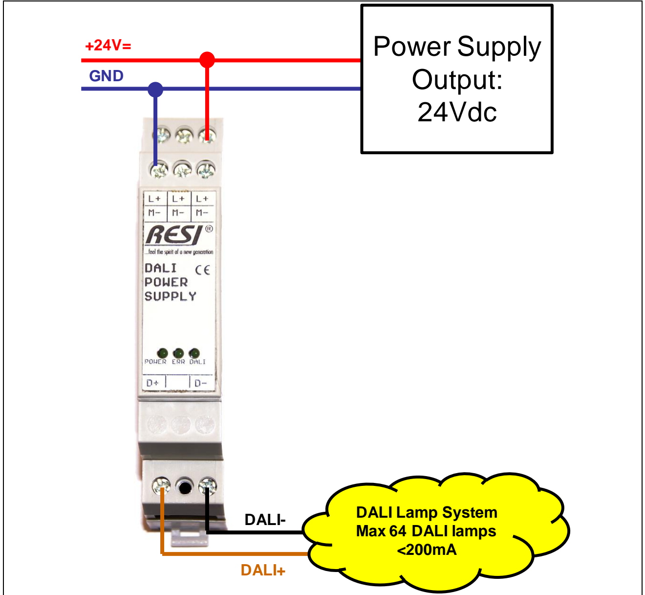
Illustration: Wiring diagram of the RESI-DAI-PS power supply
