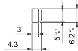
PROFILO SENSORE SENSOR PROFILE
