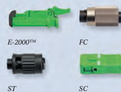
Connector housings
