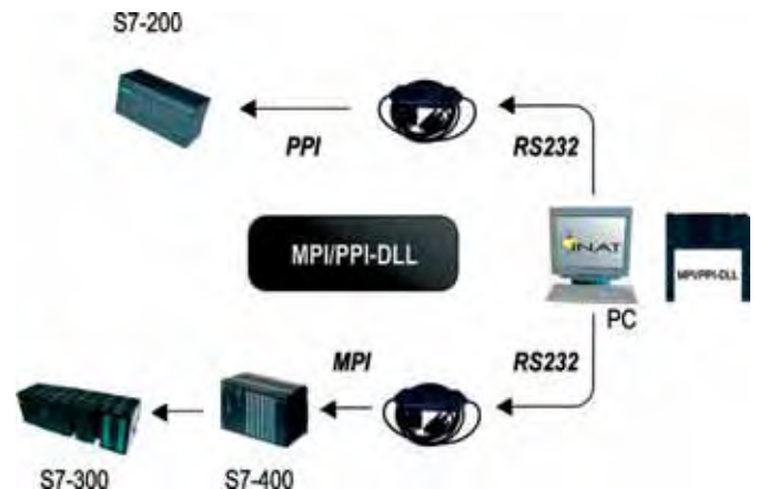
Access to S7 with MPI / PPI DLL
