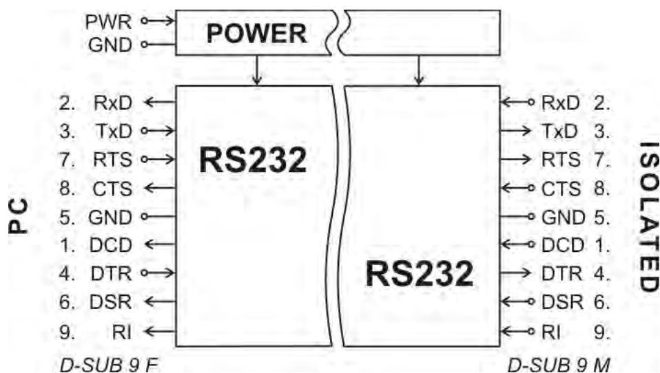
Fig. 2 – Block diagram
