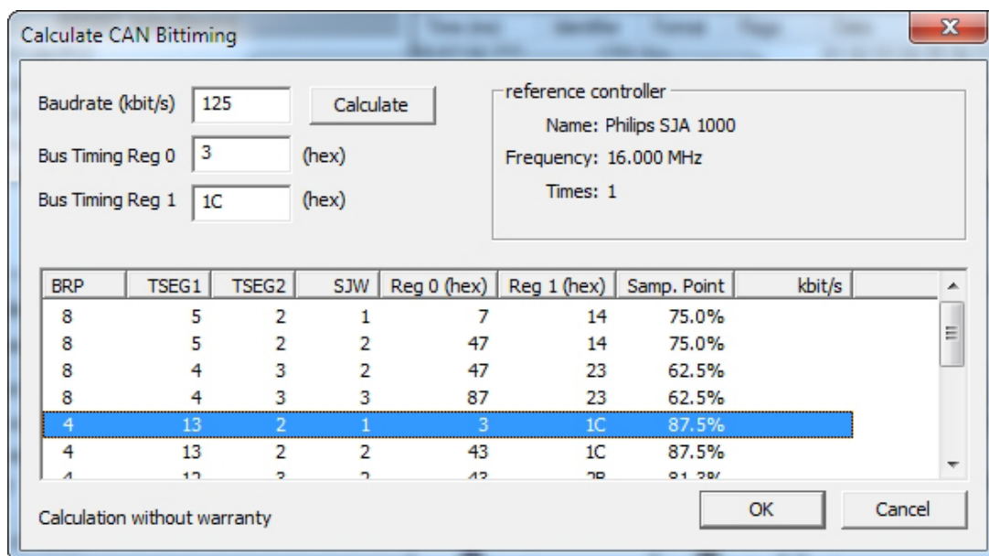
Fig. 2-6: Bit rate configuration
